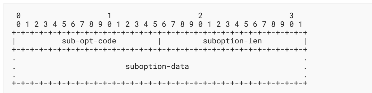
Figure 29: Vendor-Specific Options Format
