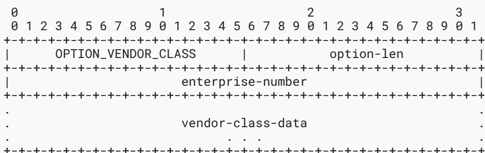
Figure 26: Vendor Class Option Format
