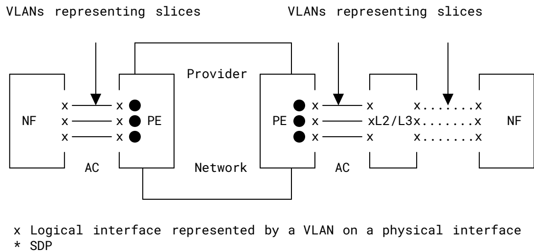
Figure 12: Example of 5G Network Slice with VLAN Handoff Providing End-to-End Connectivity
