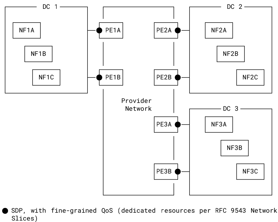
Figure 30: Example of Multi-DC Architecture
